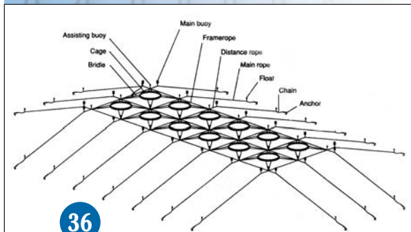
Example of a Mooring Installation
